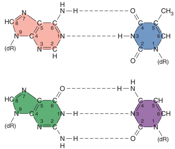
FIGURE 7-3 Normal base pairing in DNA. Top: Adenine–thymidine (A–T) pairing; bottom: guanine–cytosine (G–C) pair. Hydrogen bonds are indicated by dotted lines . Note that the G–C pairing shares three sets of hydrogen bonds, but the A–T pairing has only two. Consequently, a G–C interaction is stronger than an A–T interaction. dR, deoxyribose of the sugar-phosphate DNA backbone.
