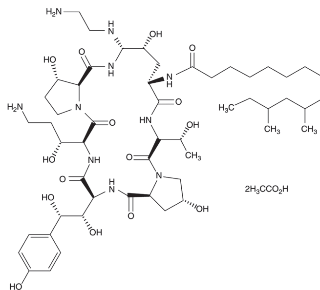
FIGURE 45-31 Structure of Caspofungin.
