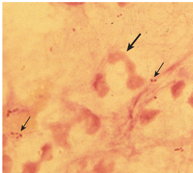
FIGURE 18-1 Gram-stain of H. influenzae in sputum. The organisms are very small ( 0.3 \times 1 \mu\text{m} ), Gram-negative coccobacilli (small arrows). The large, irregularly shaped objects (large arrow) are the nuclei of polymorphonuclear cells. Mucus is faintly stained pink in the background.
