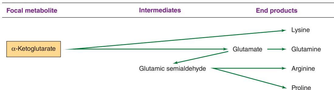
FIGURE 6-5 Biosynthetic end products formed from \alpha -ketoglutarate.
