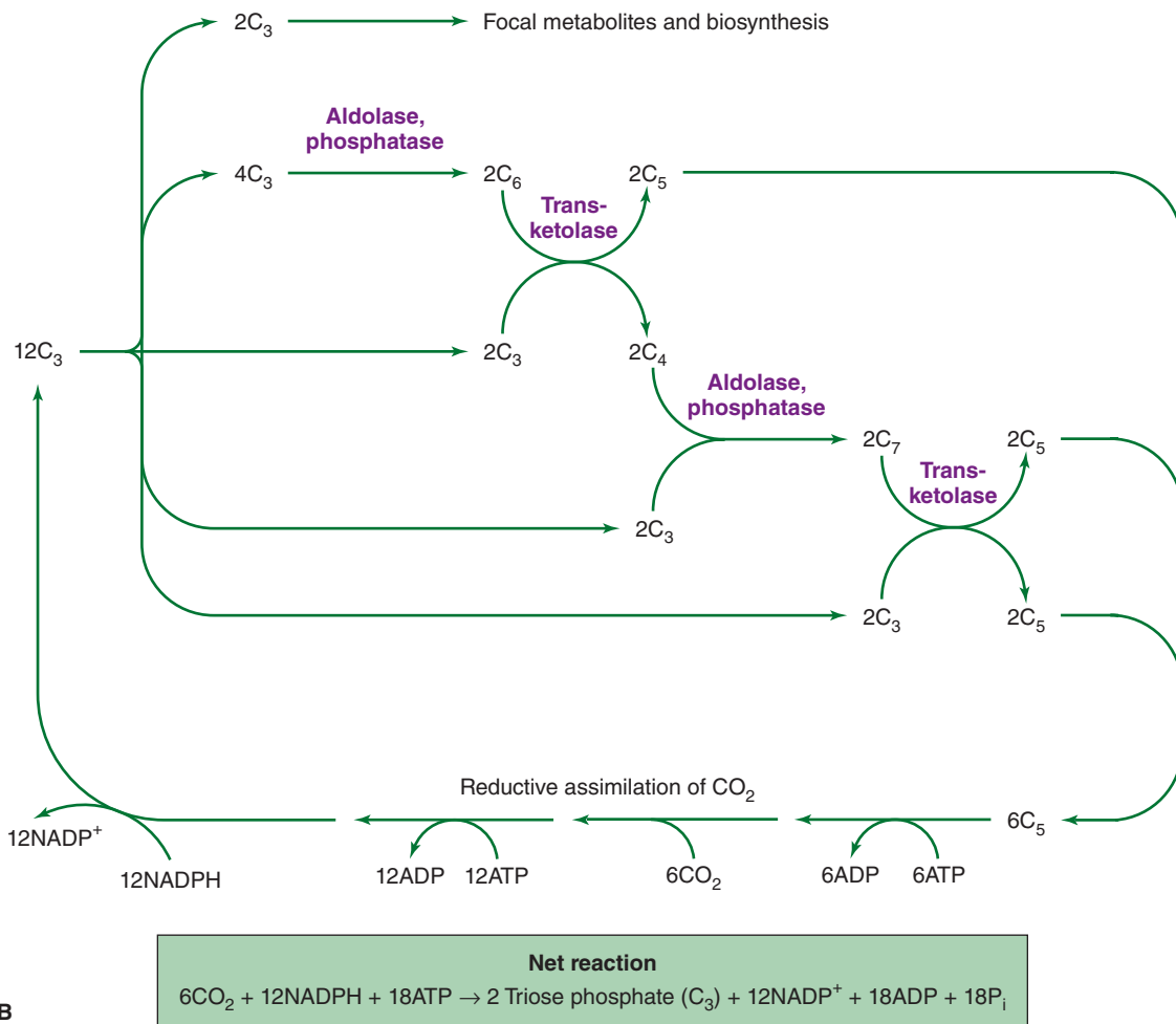
FIGURE 6-13 The Calvin cycle. A: Reductive assimilation of \text{CO}_2 . Adenosine triphosphate (ATP) and NADPH (nicotinamide adenine dinucleotide phosphate) are used to reductively convert pentose 5-phosphate ( \text{C}_5 ) to two molecules of triose phosphate ( \text{C}_3 ). B: The Calvin cycle is completed by carbohydrate rearrangement reactions (Figure 6-6) that allow the net synthesis of carbohydrate and the regeneration of pentose phosphate so that the cycle may continue. ADP, adenosine diphosphate.
