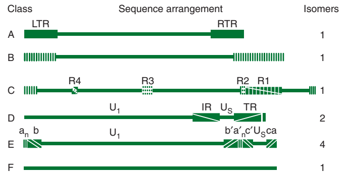
FIGURE 33-1 Schematic diagram of sequence arrangements of herpesviruses DNAs. Genome classes A, B, C, D, E, and F are exemplified by channel catfish virus, herpesvirus saimiri, Epstein-Barr virus, varicella-zoster virus, herpes simplex viruses, and tupaia herpesvirus, respectively. Horizontal lines represent unique regions. Reiterated domains are shown as rectangles : left and right terminal repeats (LTR and RTR) for class A; repeats R1–R4 for internal repeats of class C; and internal and terminal repeats (IR and TR) of class D. In class B, terminal sequences are reiterated numerous times at both termini. The termini of class E consist of two elements. The terminal sequences (ab and ca) are inserted in an inverted orientation separating the unique sequences into long (U 1 ) and short (U s ) domains. Genomes of class F have no terminal repetitions. The components of the genomes in classes D and E invert. In class D (varicella-zoster virus), the short component inverts relative to the long, and the DNA forms two populations (isomers) differing in the orientation of the short component. In class E (herpes simplex virus), both the short and long components can invert, and viral DNA consists of four isomers. (Reproduced with permission from Roizman B: Herpesviridae: A brief introduction. In Fields BN, Knipe DM [editors-in-chief]. Virology , 2nd ed. Raven Press, 1990, pp. 1787–1793.)
